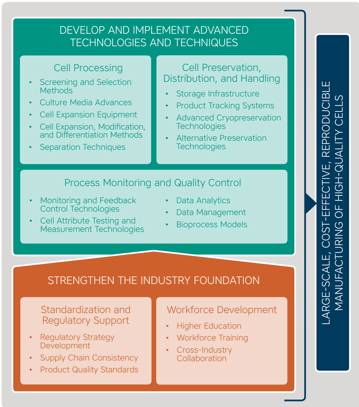
Figure 2. Roadmap Strategy
